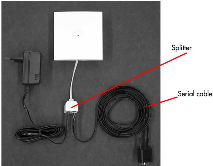
Figure 18 KIRK Programming Kit Repeater
